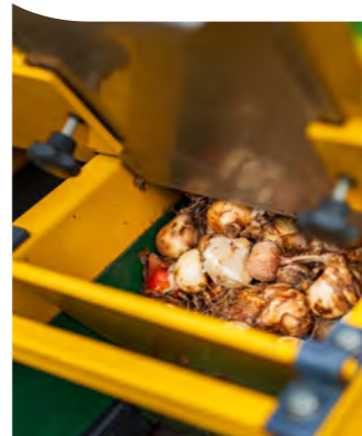
Bulbs are conveyed via a conveyor belt to the planting feet
